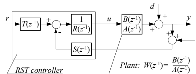
Fig.1 RST control structure
