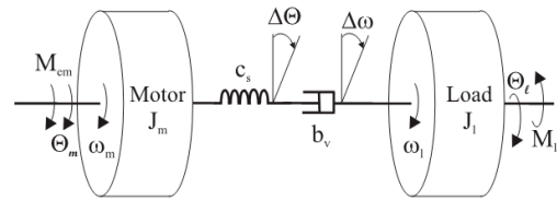
Fig. 2. Flexible coupling of motor axle and load
