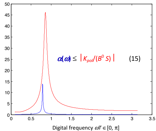
Fig.3. Illustration of the robust stability test
