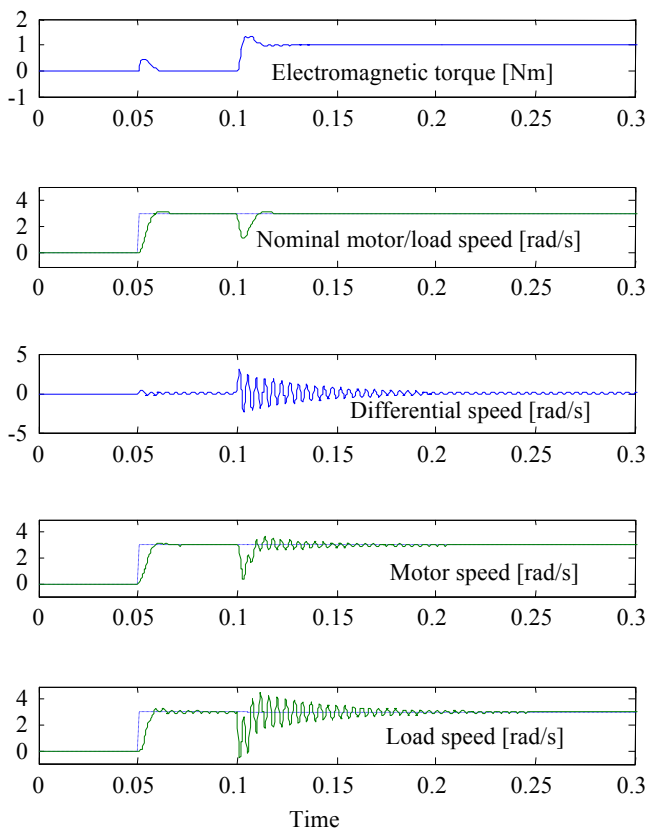
Fig.4. Simulation of the RST controller design efficiency
